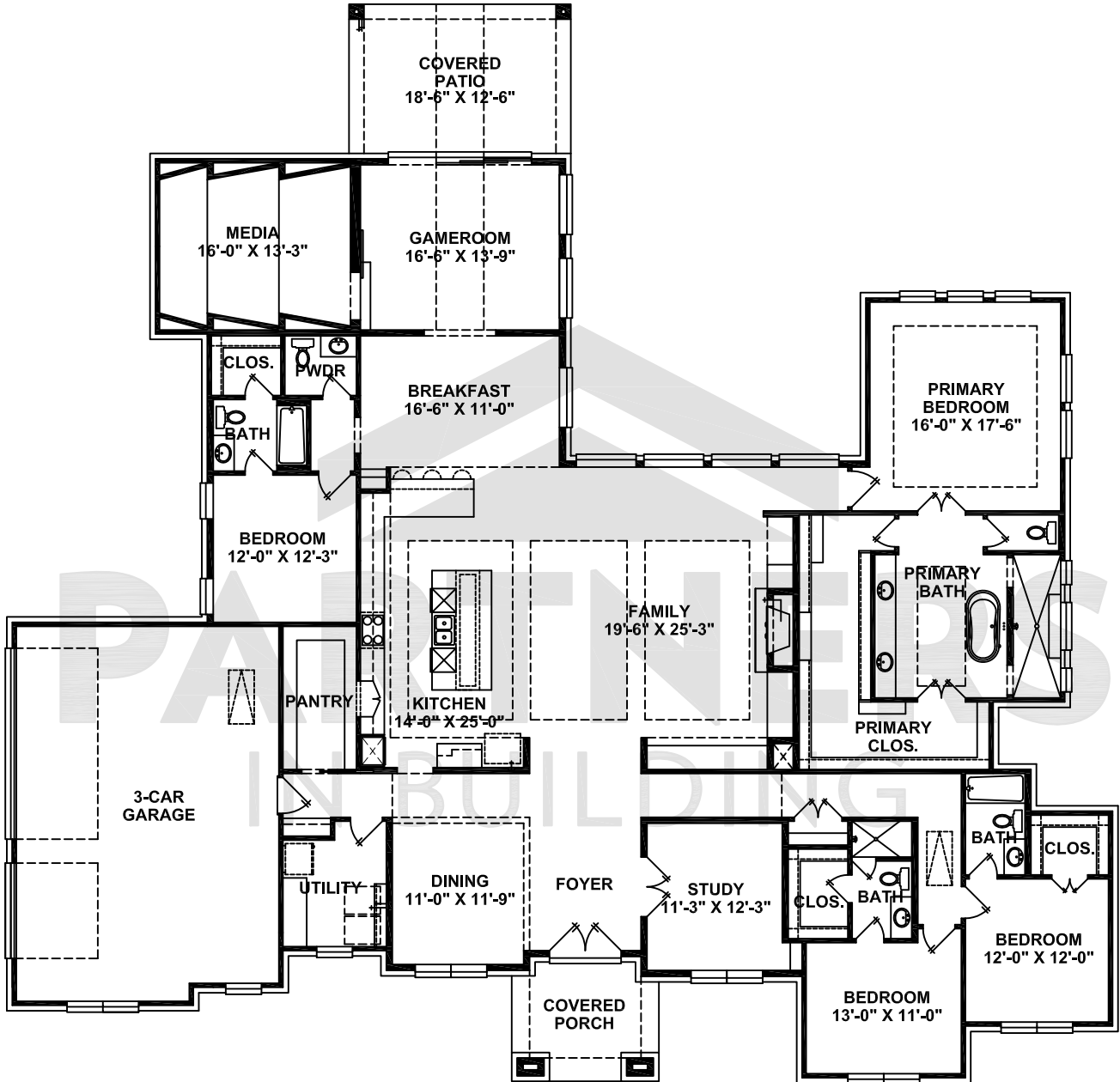
FIRST FLOOR
