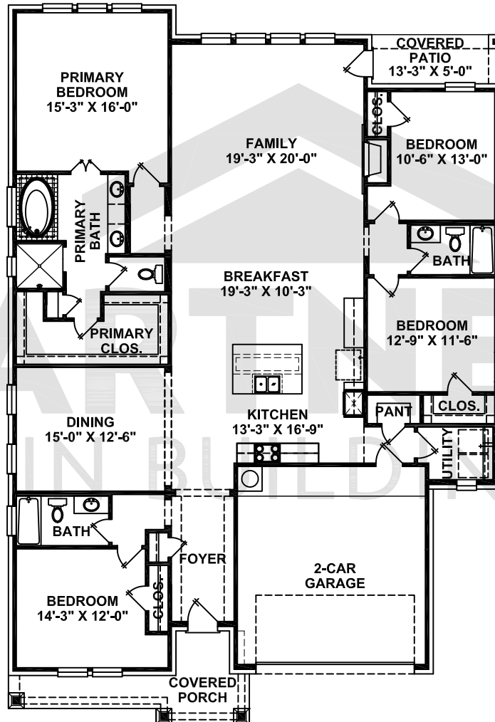
FIRST FLOOR
