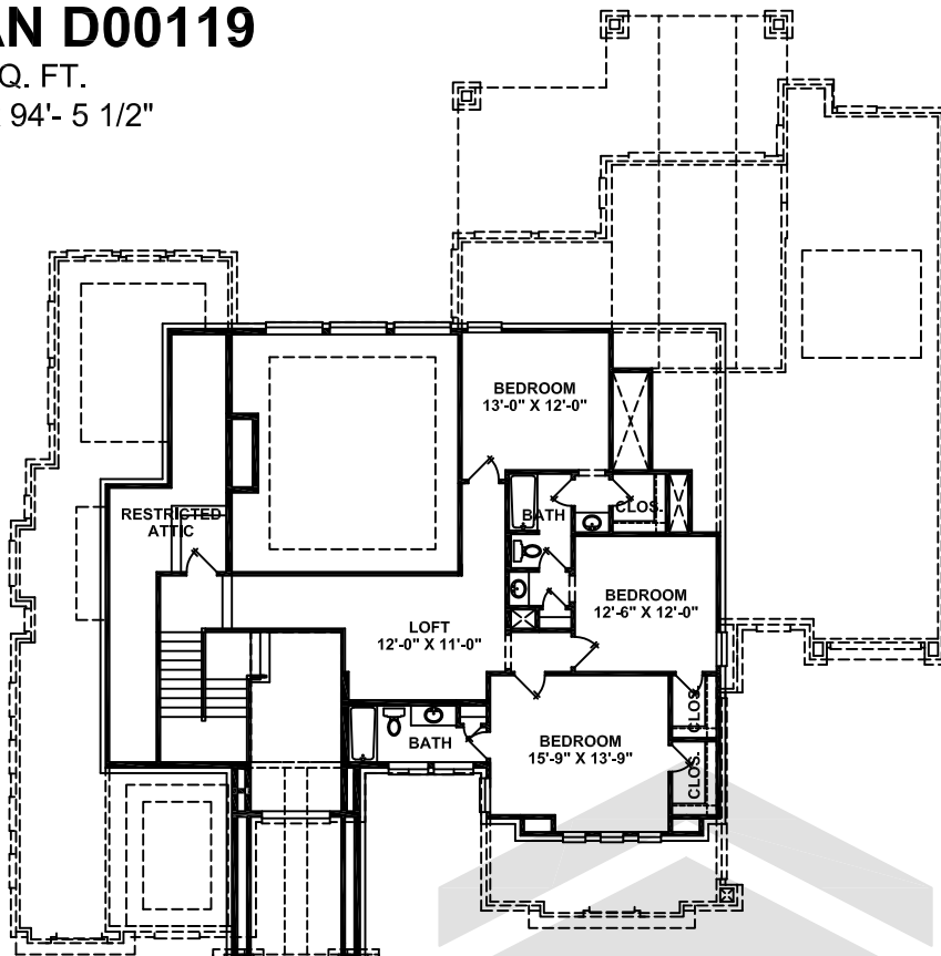
SECOND FLOOR
