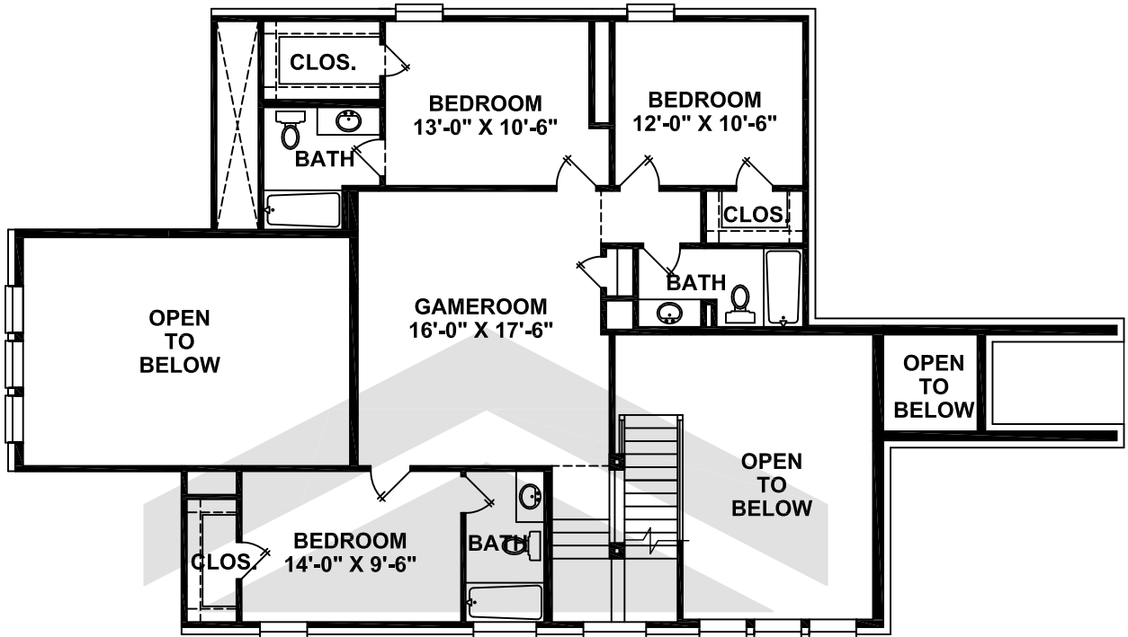
SECOND FLOOR
