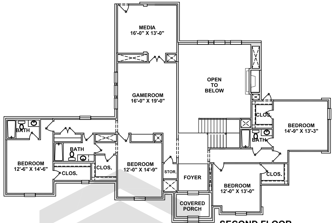
SECOND FLOOR
