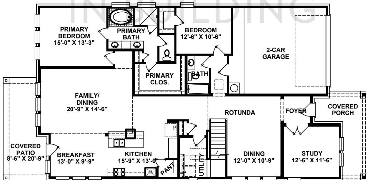
FIRST FLOOR
