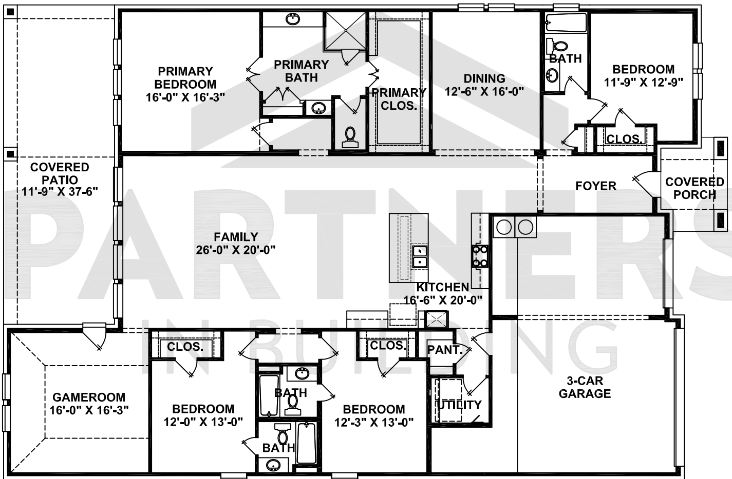
FIRST FLOOR
