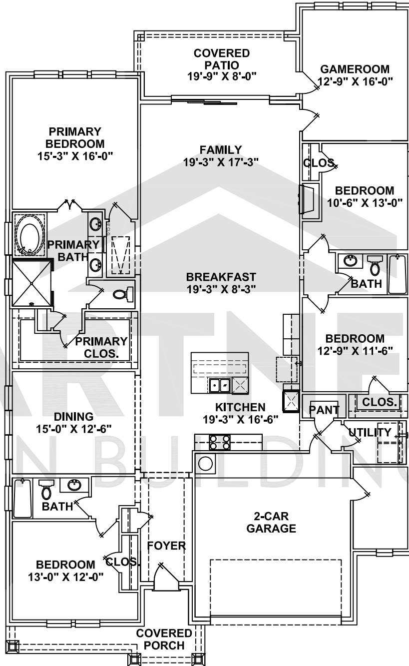
FIRST FLOOR
