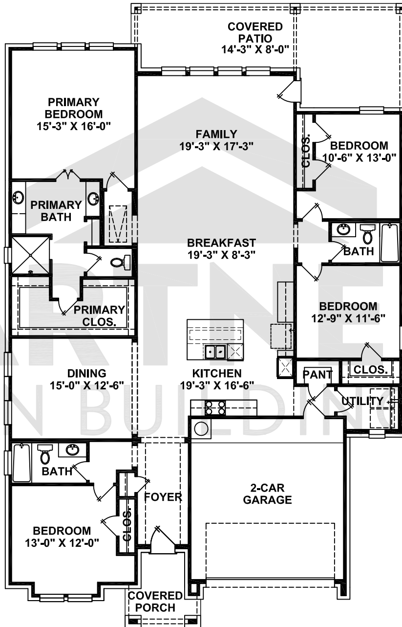
FIRST FLOOR
