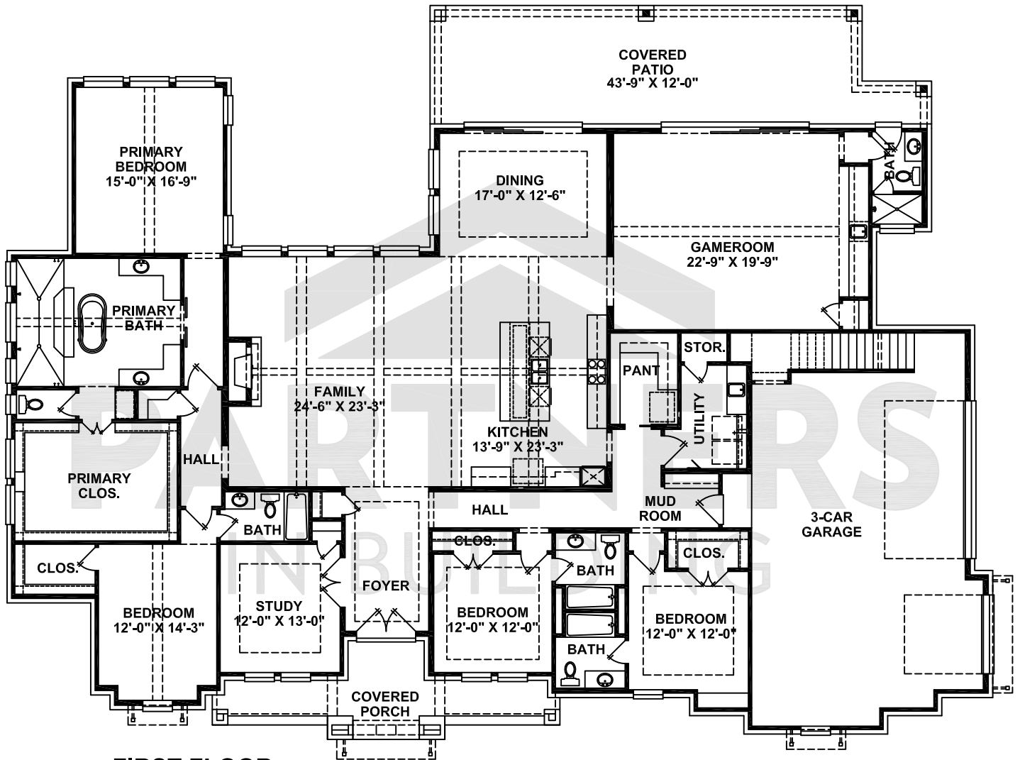
FIRST FLOOR
