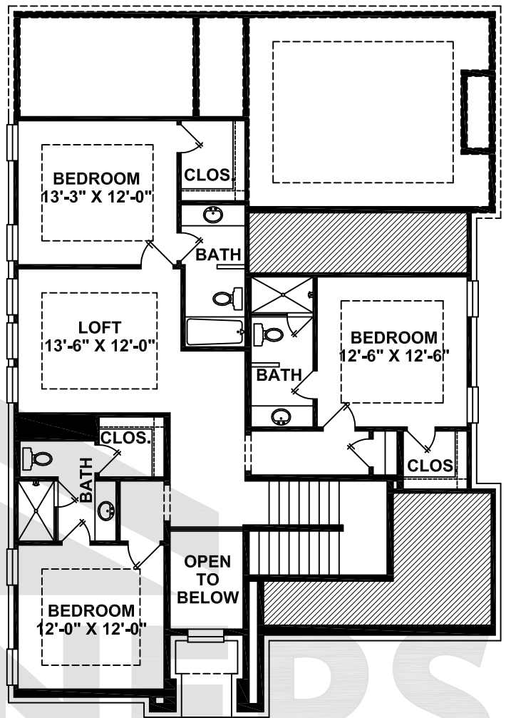
SECOND FLOOR
