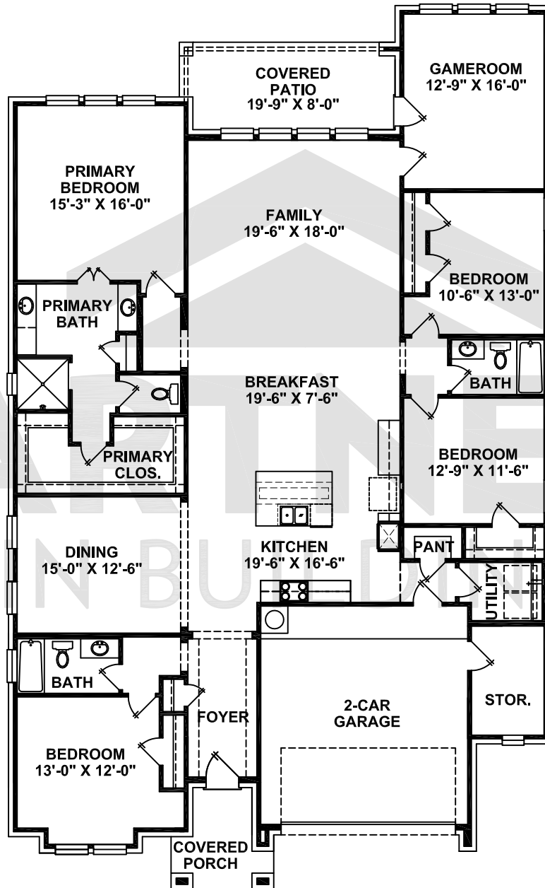
FIRST FLOOR
