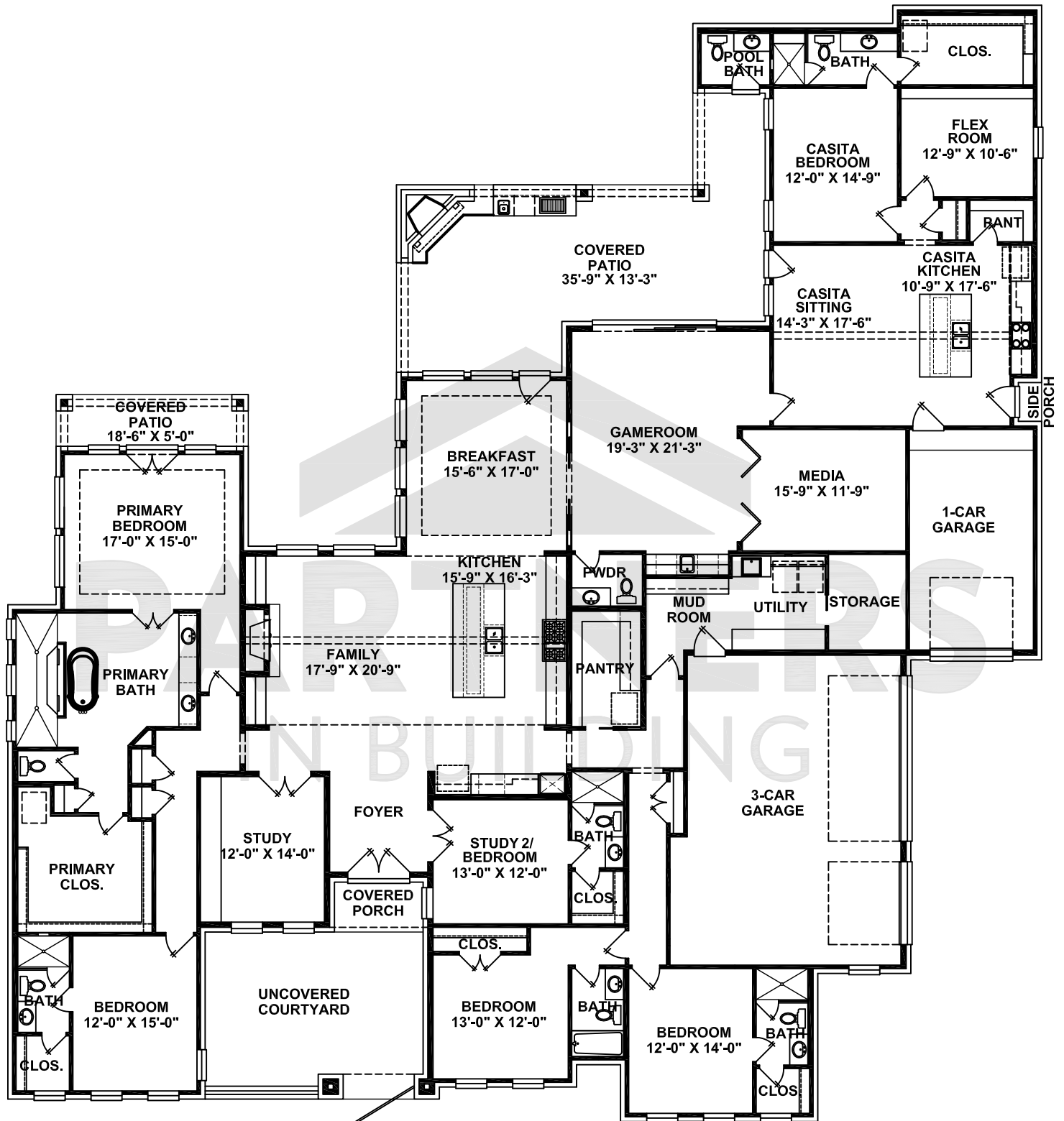
FIRST FLOOR
