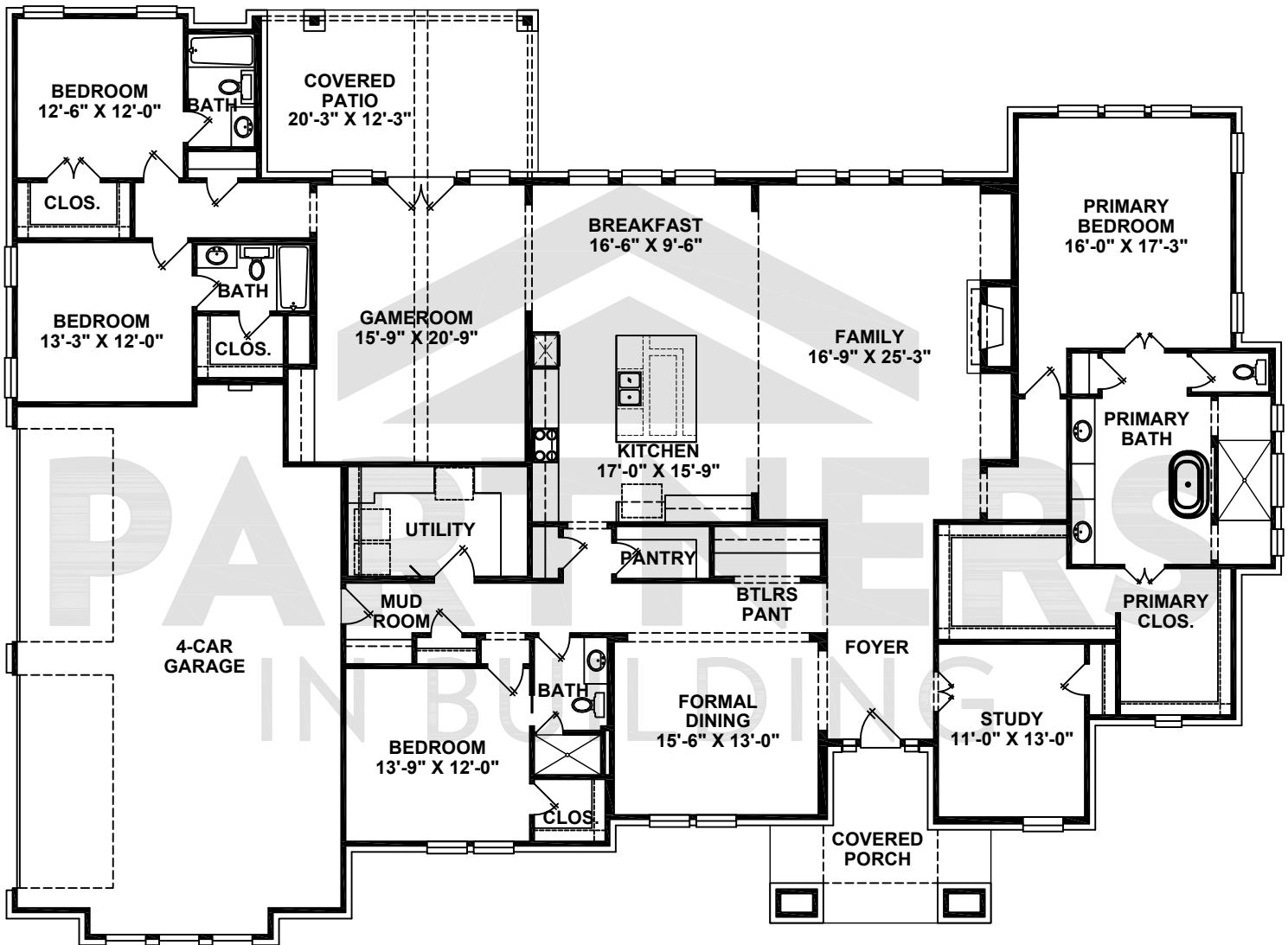
FIRST FLOOR
