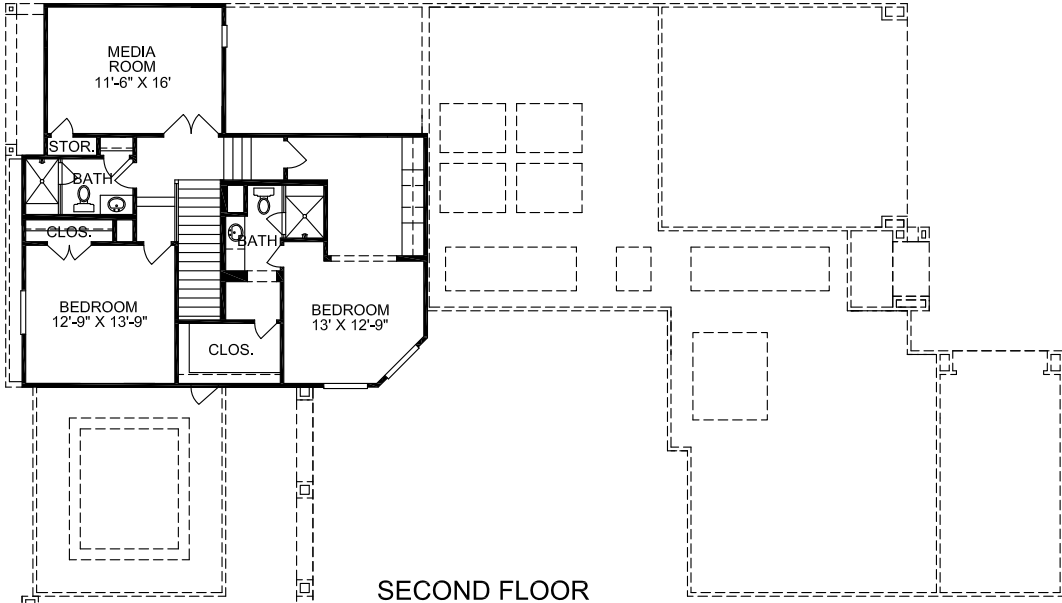
SECOND FLOOR
